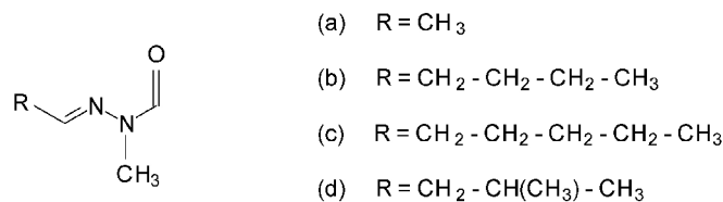
Figure 2. Structures of toxic compounds in fresh false morel ( Gyromitra esculenta ). (a) Acetaldehyde N-methyl-N-formyl hydrazone (gyromitrin), (b) pentanal N-methyl-N-formyl hydrazone, (c) hexanal N-methyl-N-formyl hydrazone, (d) 3-methylbutanal N-methyl-N-formyl hydrazone.
